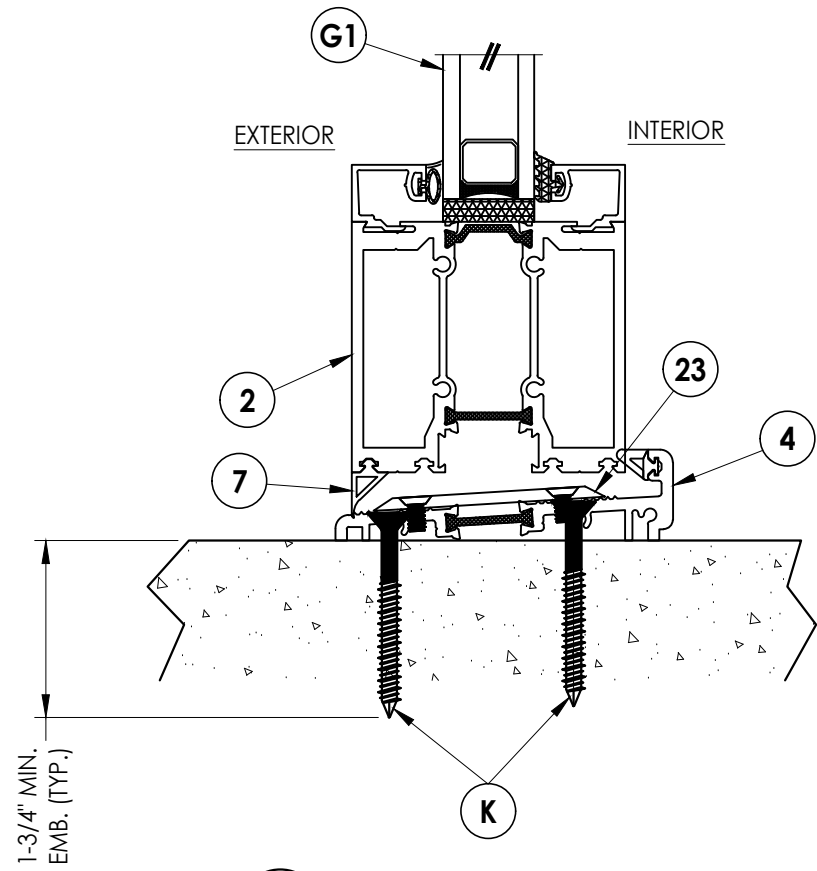
1 VERTICAL CROSS SECTION 9 OUTSWING SILL
